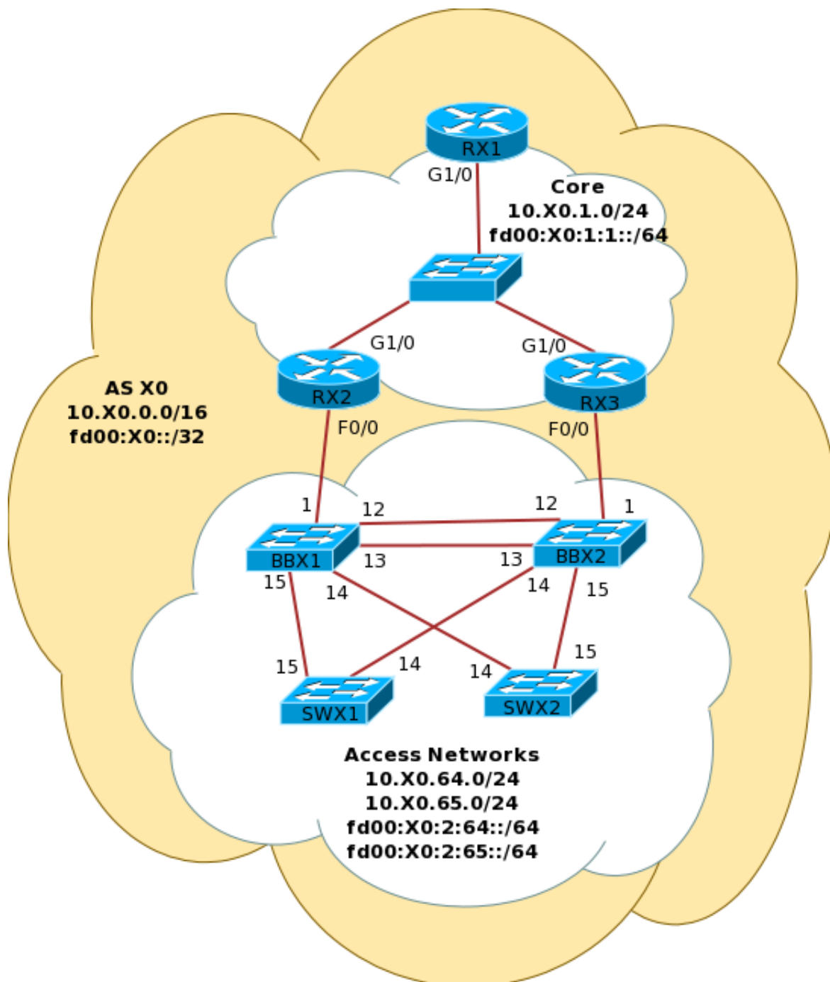
Physical Topology
