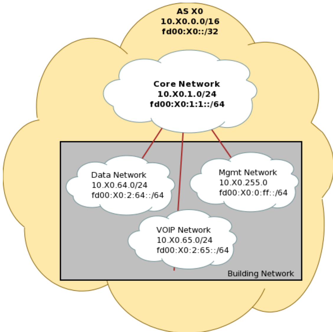
Logical Topology
